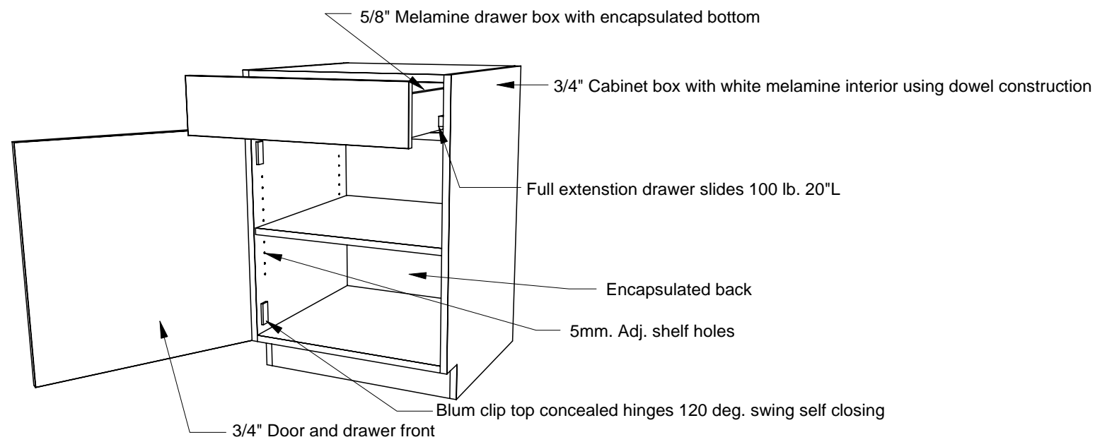
BASE CABINET
