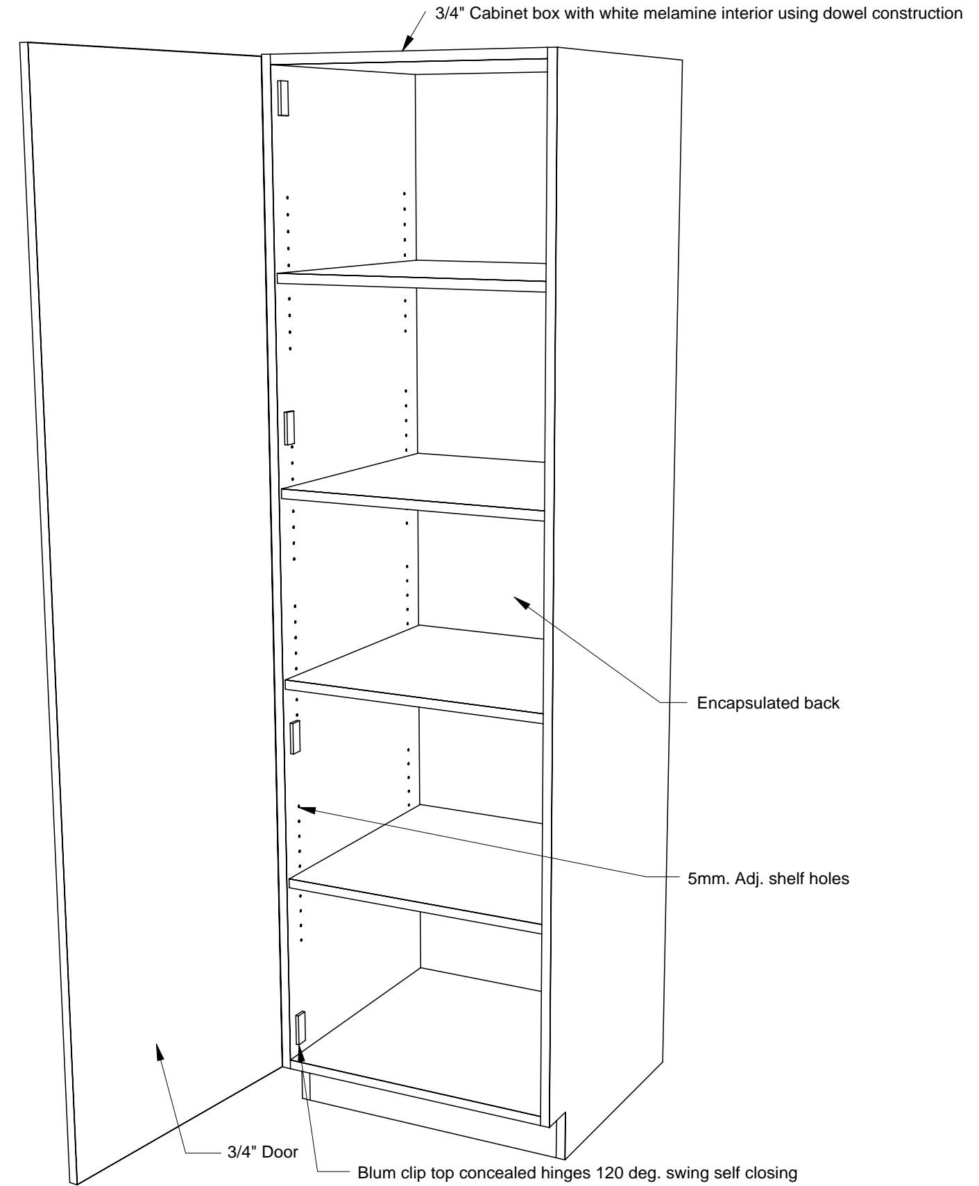
TALL CABINET
