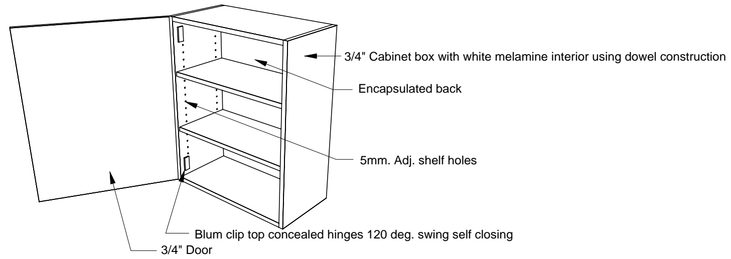
UPPER WALL CABINET
