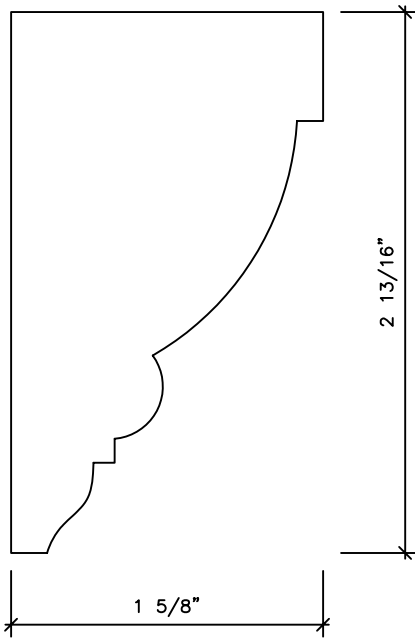
AC6011 1 5/8 x 2 13/16
