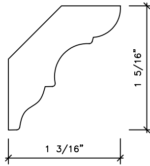
AC6014 5/8 x 1 13/16
