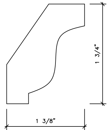
AC6010 3/4 x 2 1/4
