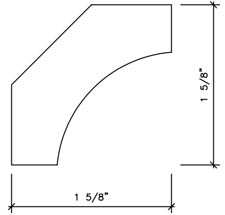
AC6008 7/8 x 2 3/8
