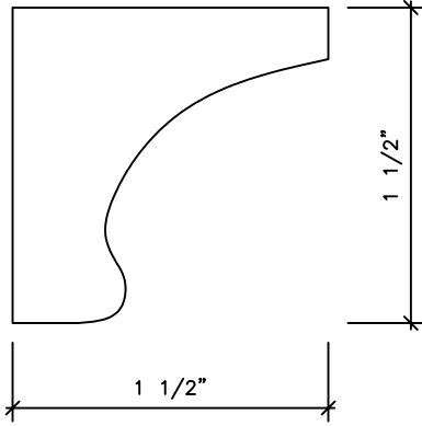
AC6002 1 1/2 x 1 1/2
