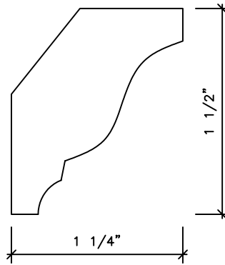
AC6007 3/4 x 2
