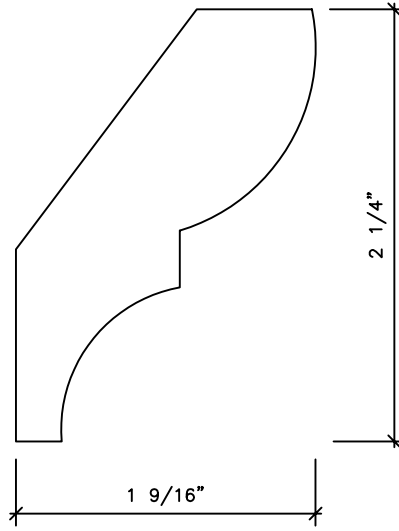
AC6005 1 x 2 3/4
