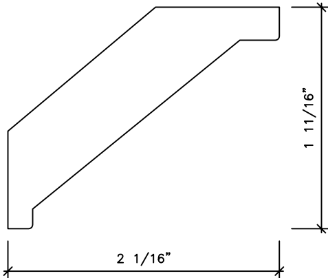
AC6004 3/4 x 2 5/8
