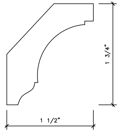
AC6009 3/4 x 2 3/8
